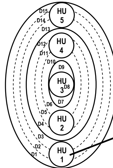
One 15-Dimensional Matrix with 5 Harmonic Universes
